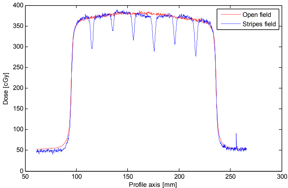
Figure 2 Profiles of an open field (red) and dynamic stripes field (blue).
